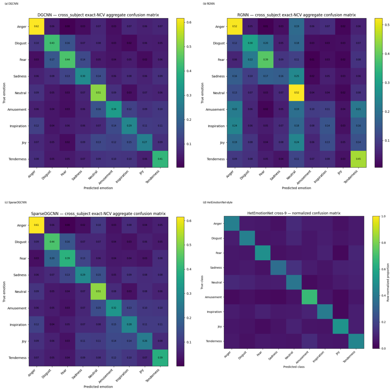
Fig. 4. Row-normalized aggregate confusion matrices from both completed notebooks.
